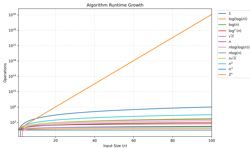
Figure 2.1: Visual comparison of common running time growth rates.
